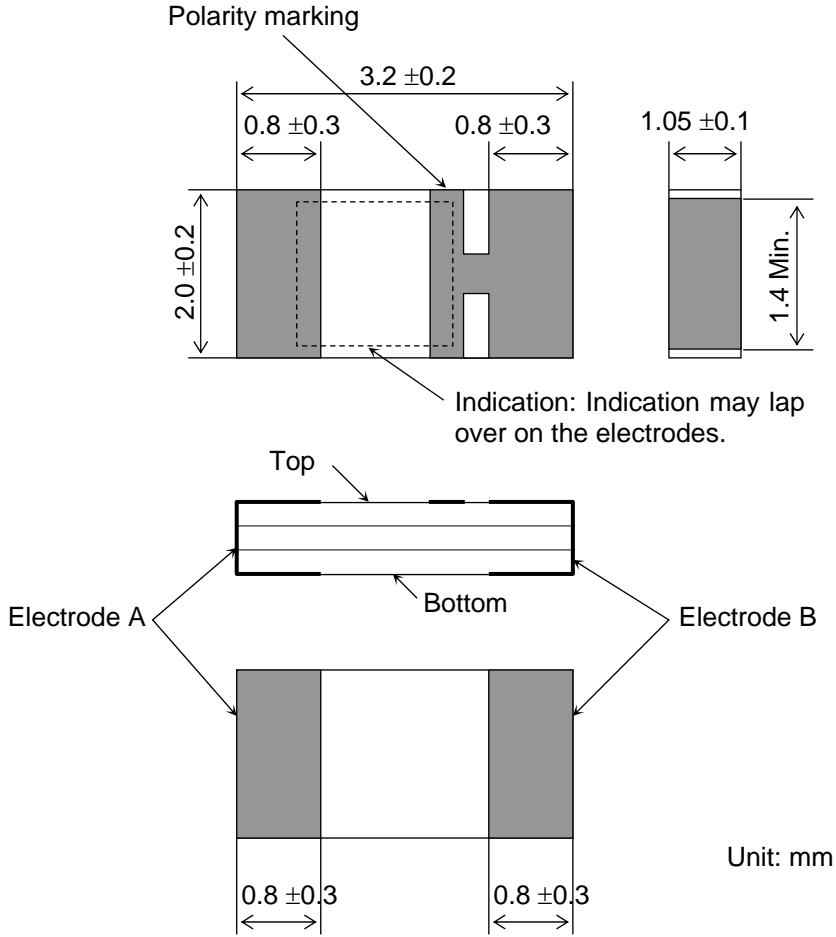
Figure 2. Dimensions
